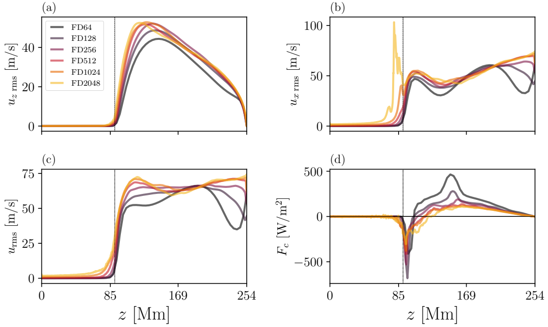
Figure 3. Vertical profiles of the (a) vertical; (b) horizontal; (c) total rms velocities; and (d) the convective heat flux, F_c = \rho_a c_p \langle u_z \Theta' \rangle for simulations FD64-FD2048. Different resolutions are represented by different colors indicated in panel (a).
