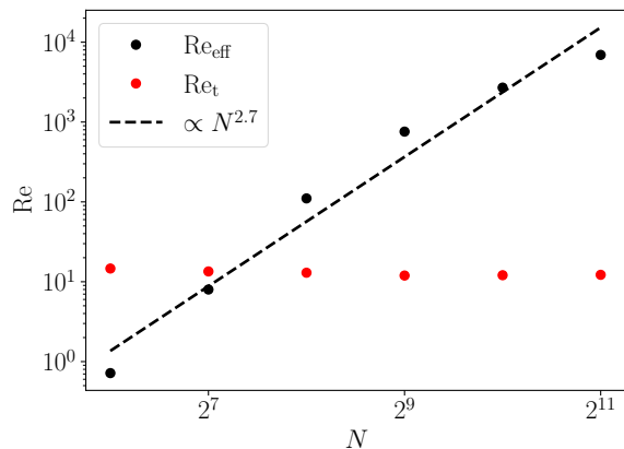
Figure 8. Effective Reynolds number (black points) and turbulent Reynolds (red) number as a function of the resolution. The black dashed line shows a fitted power law as indicated in the legend.
