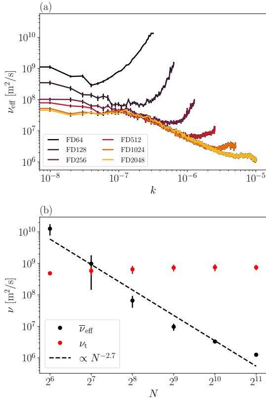
Figure 7. (a) Effective numerical viscosity as a function of the wave number, k , for simulations with different resolutions; (b) effective numerical viscosity (black points) of the smallest resolved scales and turbulent viscosity (red) versus the resolution, N . Upper and bottom panels show vertical error bars multiplied by a factors of 2 and 10, respectively, to make them noticeable. The black dashed line shows a fitted power law as indicated in the legend.
