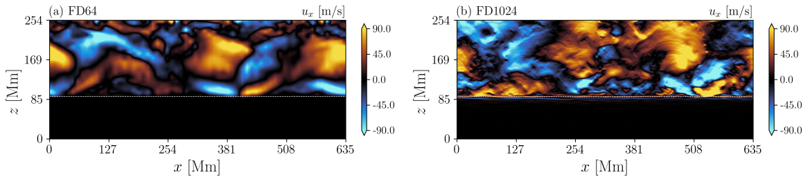
Figure 4. Snapshots of horizontal velocities for simulations (a) FD64, and (b) FD1024. Yellow (blue) contours indicate horizontal flow towards the right (left).
